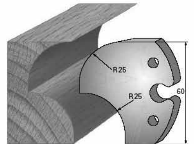
SP-Messer/Blade = Art.-Nr./Item no. 60011 HS-Messer/Blade = Art.-Nr./Item no. 62011 Abweiser/Deflector = Art.-Nr./Item no. 61011A
