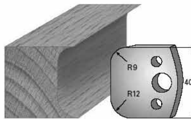
SP-Messer/Blade = Art.-Nr./Item no. 3650 HS-Messer/Blade = Art.-Nr./Item no. 36350 Abweiser/Deflector = Art.-Nr./Item no. 3750
