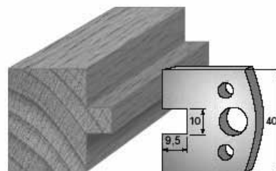
SP-Messer/Blade = Art.-Nr./Item no. 3692 HS-Messer/Blade = Art.-Nr./Item no. 36392 Abweiser/Deflector = Art.-Nr./Item no. 3792
