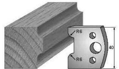
SP-Messer/Blade = Art.-Nr./Item no. 3663 HS-Messer/Blade = Art.-Nr./Item no. 36363 Abweiser/Deflector = Art.-Nr./Item no. 3763
