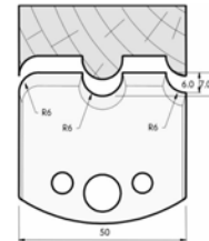
SP-Messer/Blade = Art.-Nr./Item no. 38534 HS-Messer/Blade = Art.-Nr./Item no. 36534 Abweiser/Deflector = Art.-Nr./Item no. 39534
