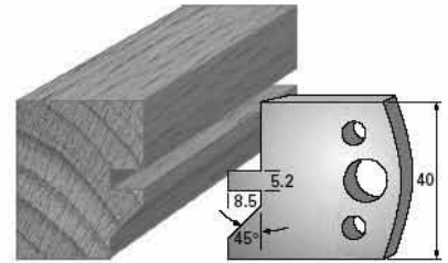
SP-Messer/Blade = Art.-Nr./Item no. 3684 HS-Messer/Blade = Art.-Nr./Item no. 36384 Abweiser/Deflector = Art.-Nr./Item no. 3784
