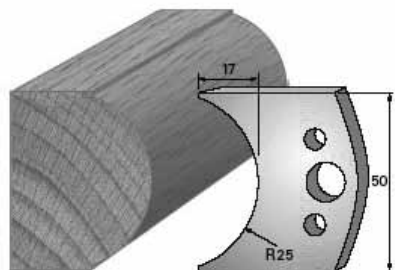
SP-Messer/Blade = Art.-Nr./Item no. 38546 HS-Messer/Blade = Art.-Nr./Item no. 36546 Abweiser/Deflector = Art.-Nr./Item no. 39546
