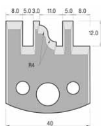
SP-Messer/Blade = Art.-Nr./Item no. 36136 HS-Messer/Blade = Art.-Nr./Item no. 36436 Abweiser/Deflector = Art.-Nr./Item no. 37136
