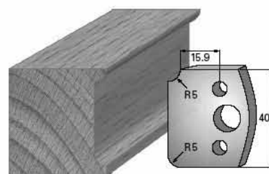
SP-Messer/Blade = Art.-Nr./Item no. 36172 HS-Messer/Blade = Art.-Nr./Item no. 36472 Abweiser/Deflector = Art.-Nr./Item no. 37172
