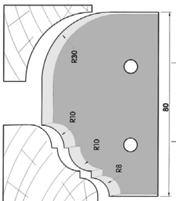
HS-Messer/Blade = Art.-Nr./Item no. 80004 Abweiser/Deflector = Art.-Nr./Item no. 81004
