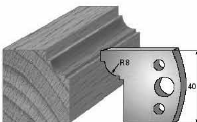
SP-Messer/Blade = Art.-Nr./Item no. 3667 HS-Messer/Blade = Art.-Nr./Item no. 36367 Abweiser/Deflector = Art.-Nr./Item no. 3767
