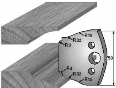
SP-Messer/Blade = Art.-Nr./Item no. 38568 HS-Messer/Blade = Art.-Nr./Item no. 36568 Abweiser/Deflector = Art.-Nr./Item no. 39568
