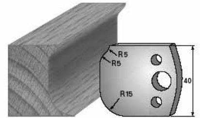
SP-Messer/Blade = Art.-Nr./Item no. 3660 HS-Messer/Blade = Art.-Nr./Item no. 36360 Abweiser/Deflector = Art.-Nr./Item no. 3760
