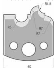
SP-Messer/Blade = Art.-Nr./Item no. 36140 HS-Messer/Blade = Art.-Nr./Item no. 36440 Abweiser/Deflector = Art.-Nr./Item no. 37140
