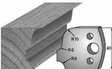
SP-Messer/Blade = Art.-Nr./Item no. 3664 HS-Messer/Blade = Art.-Nr./Item no. 36364 Abweiser/Deflector = Art.-Nr./Item no. 3764
