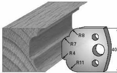
SP-Messer/Blade = Art.-Nr./Item no. 3623 HS-Messer/Blade = Art.-Nr./Item no. 36323 Abweiser/Deflector = Art.-Nr./Item no. 3723
