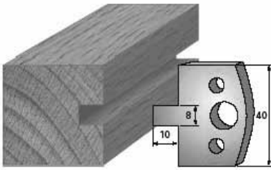
SP-Messer/Blade = Art.-Nr./Item no. 3694 HS-Messer/Blade = Art.-Nr./Item no. 36394 Abweiser/Deflector = Art.-Nr./Item no. 3794
