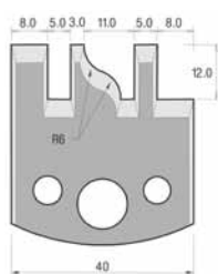
SP-Messer/Blade = Art.-Nr./Item no. 36138 HS-Messer/Blade = Art.-Nr./Item no. 36438 Abweiser/Deflector = Art.-Nr./Item no. 37138
