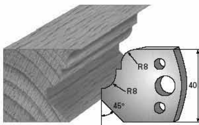
SP-Messer/Blade = Art.-Nr./Item no. 3673 HS-Messer/Blade = Art.-Nr./Item no. 36373 Abweiser/Deflector = Art.-Nr./Item no. 3773
