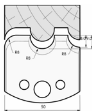
SP-Messer/Blade = Art.-Nr./Item no. 38536 HS-Messer/Blade = Art.-Nr./Item no. 36536 Abweiser/Deflector = Art.-Nr./Item no. 39536
