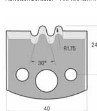
SP-Messer/Blade = Art.-Nr./Item no. 36141 HS-Messer/Blade = Art.-Nr./Item no. 36441 Abweiser/Deflector = Art.-Nr./Item no. 37141
