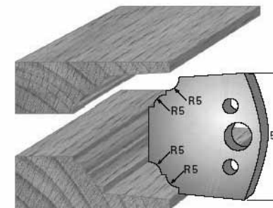
SP-Messer/Blade = Art.-Nr./Item no. 38580 HS-Messer/Blade = Art.-Nr./Item no. 36580 Abweiser/Deflector = Art.-Nr./Item no. 39580
