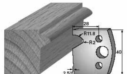
SP-Messer/Blade = Art.-Nr./Item no. 36135 HS-Messer/Blade = Art.-Nr./Item no. 36435 Abweiser/Deflector = Art.-Nr./Item no. 37135
