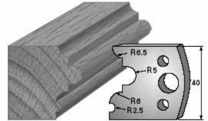
SP-Messer/Blade = Art.-Nr./Item no. 3636 HS-Messer/Blade = Art.-Nr./Item no. 36336 Abweiser/Deflector = Art.-Nr./Item no. 3736
