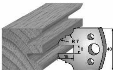
SP-Messer/Blade = Art.-Nr./Item no. 3699 - Konter 4 HS-Messer/Blade = Art.-Nr./Item no. 36399 Abweiser/Deflector = Art.-Nr./Item no. 3799
