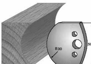
SP-Messer/Blade = Art.-Nr./Item no. 38544 HS-Messer/Blade = Art.-Nr./Item no. 36544 Abweiser/Deflector = Art.-Nr./Item no. 39544
