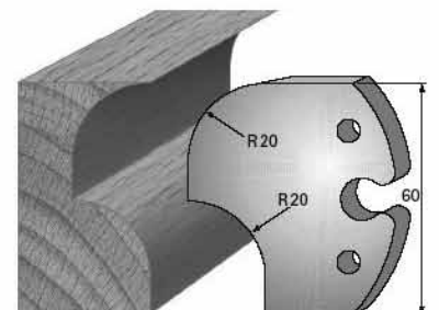
SP-Messer/Blade = Art.-Nr./Item no. 60019 HS-Messer/Blade = Art.-Nr./Item no. 62019 Abweiser/Deflector = Art.-Nr./Item no. 61019A
