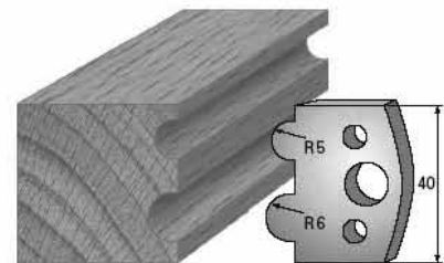
SP-Messer/Blade = Art.-Nr./Item no. 3630 HS-Messer/Blade = Art.-Nr./Item no. 36330 Abweiser/Deflector = Art.-Nr./Item no. 3730
