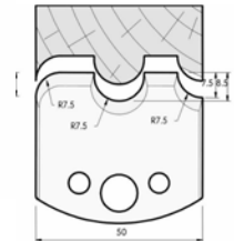
SP-Messer/Blade = Art.-Nr./Item no. 38535 HS-Messer/Blade = Art.-Nr./Item no. 36535 Abweiser/Deflector = Art.-Nr./Item no. 39535
