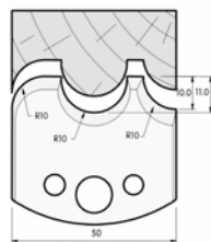
SP-Messer/Blade = Art.-Nr./Item no. 38537 HS-Messer/Blade = Art.-Nr./Item no. 36537 Abweiser/Deflector = Art.-Nr./Item no. 39537
