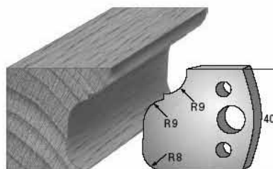
SP-Messer/Blade = Art.-Nr./Item no. 3668 HS-Messer/Blade = Art.-Nr./Item no. 36368 Abweiser/Deflector = Art.-Nr./Item no. 3768
