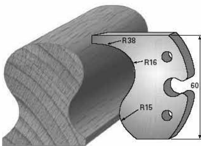
SP-Messer/Blade = Art.-Nr./Item no. 60004 HS-Messer/Blade = Art.-Nr./Item no. 62004 Abweiser/Deflector = Art.-Nr./Item no. 61004A
