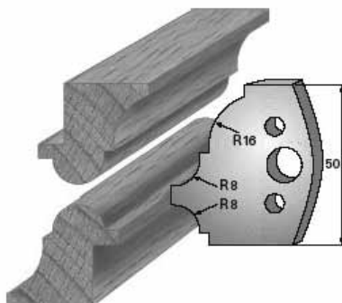
SP-Messer/Blade = Art.-Nr./Item no. 38541 HS-Messer/Blade = Art.-Nr./Item no. 36541 Abweiser/Deflector = Art.-Nr./Item no. 39541
