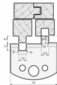
SP-Messer/Blade = Art.-Nr./Item no. 38533 HS-Messer/Blade = Art.-Nr./Item no. 36533 Abweiser/Deflector = Art.-Nr./Item no. 39533
