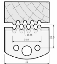
SP-Messer/Blade = Art.-Nr./Item no. 38532 HS-Messer/Blade = Art.-Nr./Item no. 36532 Abweiser/Deflector = Art.-Nr./Item no. 39532
