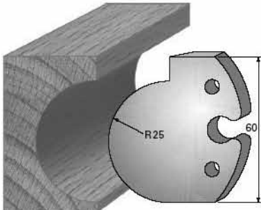
SP-Messer/Blade = Art.-Nr./Item no. 60009 HS-Messer/Blade = Art.-Nr./Item no. 62009 Abweiser/Deflector = Art.-Nr./Item no. 61009A
