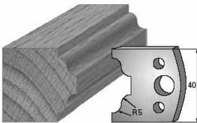
SP-Messer/Blade = Art.-Nr./Item no. 3625 HS-Messer/Blade = Art.-Nr./Item no. 36325 Abweiser/Deflector = Art.-Nr./Item no. 3725
