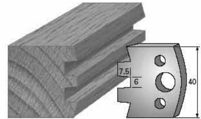
SP-Messer/Blade = Art.-Nr./Item no. 36114 HS-Messer/Blade = Art.-Nr./Item no. 36414 Abweiser/Deflector = Art.-Nr./Item no. 37114
