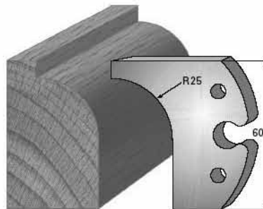
SP-Messer/Blade = Art.-Nr./Item no. 60010 HS-Messer/Blade = Art.-Nr./Item no. 62010 Abweiser/Deflector = Art.-Nr./Item no. 61010A
