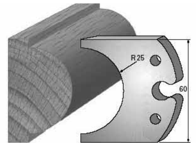
SP-Messer/Blade = Art.-Nr./Item no. 60003 HS-Messer/Blade = Art.-Nr./Item no. 62003 Abweiser/Deflector = Art.-Nr./Item no. 61003A
