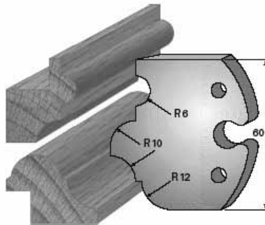
SP-Messer/Blade = Art.-Nr./Item no. 60001 HS-Messer/Blade = Art.-Nr./Item no. 62001 Abweiser/Deflector = Art.-Nr./Item no. 61001A
