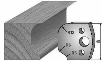
SP-Messer/Blade = Art.-Nr./Item no. 3648 HS-Messer/Blade = Art.-Nr./Item no. 36348 Abweiser/Deflector = Art.-Nr./Item no. 3748
