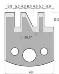
SP-Messer/Blade = Art.-Nr./Item no. 36139 HS-Messer/Blade = Art.-Nr./Item no. 36439 Abweiser/Deflector = Art.-Nr./Item no. 37139
