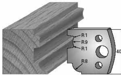
SP-Messer/Blade = Art.-Nr./Item no. 3626 HS-Messer/Blade = Art.-Nr./Item no. 36326 Abweiser/Deflector = Art.-Nr./Item no. 3726
