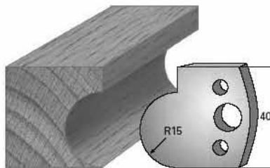
SP-Messer/Blade = Art.-Nr./Item no. 3665 HS-Messer/Blade = Art.-Nr./Item no. 36365 Abweiser/Deflector = Art.-Nr./Item no. 3765
