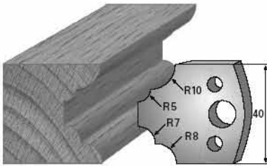
SP-Messer/Blade = Art.-Nr./Item no. 3622 HS-Messer/Blade = Art.-Nr./Item no. 36322 Abweiser/Deflector = Art.-Nr./Item no. 3722
