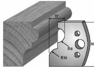
SP-Messer/Blade = Art.-Nr./Item no. 38551 HS-Messer/Blade = Art.-Nr./Item no. 36551 Abweiser/Deflector = Art.-Nr./Item no. 39551
