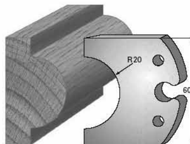
SP-Messer/Blade = Art.-Nr./Item no. 60016 HS-Messer/Blade = Art.-Nr./Item no. 62016 Abweiser/Deflector = Art.-Nr./Item no. 61016A
