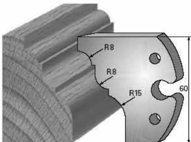
SP-Messer/Blade = Art.-Nr./Item no. 60012 HS-Messer/Blade = Art.-Nr./Item no. 62012 Abweiser/Deflector = Art.-Nr./Item no. 61012A
