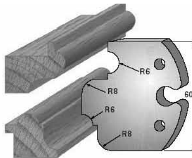
SP-Messer/Blade = Art.-Nr./Item no. 60006 HS-Messer/Blade = Art.-Nr./Item no. 62006 Abweiser/Deflector = Art.-Nr./Item no. 61006A
