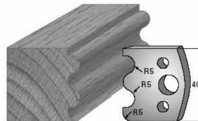
SP-Messer/Blade = Art.-Nr./Item no. 3606 HS-Messer/Blade = Art.-Nr./Item no. 36306 Abweiser/Deflector = Art.-Nr./Item no. 3706
