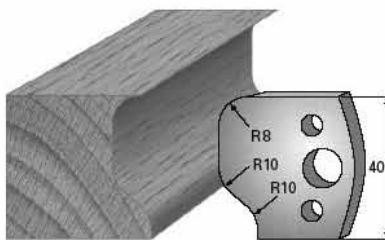
SP-Messer/Blade = Art.-Nr./Item no. 3649 HS-Messer/Blade = Art.-Nr./Item no. 36349 Abweiser/Deflector = Art.-Nr./Item no. 3749
