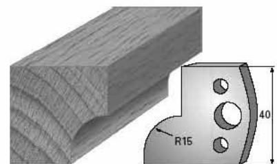
SP-Messer/Blade = Art.-Nr./Item no. 3657 HS-Messer/Blade = Art.-Nr./Item no. 36357 Abweiser/Deflector = Art.-Nr./Item no. 3757
