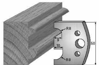
SP-Messer/Blade = Art.-Nr./Item no. 38514 HS-Messer/Blade = Art.-Nr./Item no. 36514 Abweiser/Deflector = Art.-Nr./Item no. 39514
