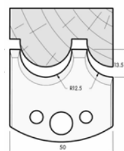
SP-Messer/Blade = Art.-Nr./Item no. 38538 HS-Messer/Blade = Art.-Nr./Item no. 36538 Abweiser/Deflector = Art.-Nr./Item no. 39538
