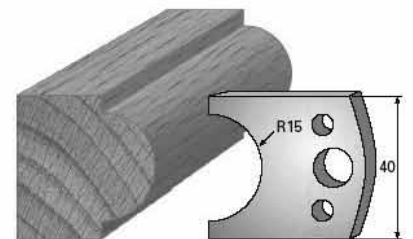
SP-Messer/Blade = Art.-Nr./Item no. 3666 HS-Messer/Blade = Art.-Nr./Item no. 36366 Abweiser/Deflector = Art.-Nr./Item no. 3766
