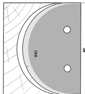
HS-Messer/Blade = Art.-Nr./Item no. 80003 Abweiser/Deflector = Art.-Nr./Item no. 81003
