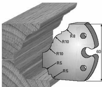
SP-Messer/Blade = Art.-Nr./Item no. 60021 HS-Messer/Blade = Art.-Nr./Item no. 62021 Abweiser/Deflector = Art.-Nr./Item no. 61021A
