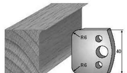
SP-Messer/Blade = Art.-Nr./Item no. 3669 HS-Messer/Blade = Art.-Nr./Item no. 36369 Abweiser/Deflector = Art.-Nr./Item no. 3769
