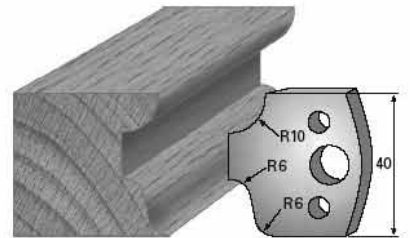
SP-Messer/Blade = Art.-Nr./Item no. 3645 HS-Messer/Blade = Art.-Nr./Item no. 36345 Abweiser/Deflector = Art.-Nr./Item no. 3745
