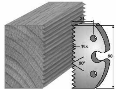
SP-Messer/Blade = Art.-Nr./Item no. 60003 HS-Messer/Blade = Art.-Nr./Item no. 62003 Abweiser/Deflector = Art.-Nr./Item no. 61003A
