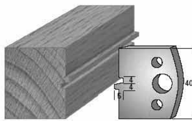
SP-Messer/Blade = Art.-Nr./Item no. 3674 HS-Messer/Blade = Art.-Nr./Item no. 36374 Abweiser/Deflector = Art.-Nr./Item no. 3774
