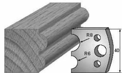
SP-Messer/Blade = Art.-Nr./Item no. 3651 HS-Messer/Blade = Art.-Nr./Item no. 36351 Abweiser/Deflector = Art.-Nr./Item no. 3751
