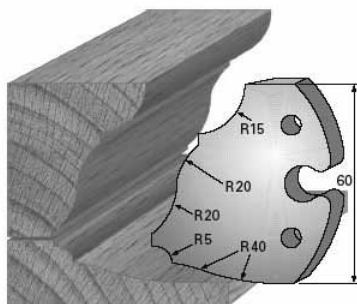
SP-Messer/Blade = Art.-Nr./Item no. 60020 HS-Messer/Blade = Art.-Nr./Item no. 62020 Abweiser/Deflector = Art.-Nr./Item no. 61020A
