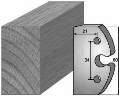
SP-Messer/Blade = Art.-Nr./Item no. 60000 HS-Messer/Blade = Art.-Nr./Item no. 62000 Abweiser/Deflector = Art.-Nr./Item no. 61000A
