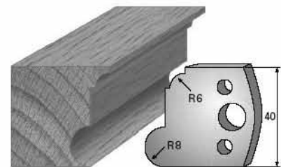
SP-Messer/Blade = Art.-Nr./Item no. 3654 HS-Messer/Blade = Art.-Nr./Item no. 36354 Abweiser/Deflector = Art.-Nr./Item no. 3754
